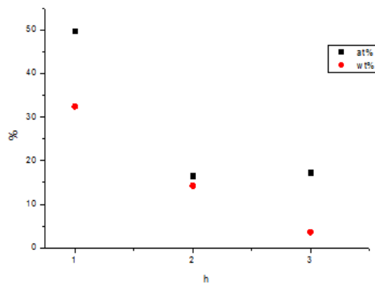
Figure 8. Results of EDX investigation of Taylor cones extracted on anode sample with power regime: U=60V , C=200\mu F , d=0,2mm , S=0.2 mm , where h1 – top, h2 – lateral surface, h3 – crater. On the graph, it is shown atomic and weight oxygen concentration in different zones of the cone
