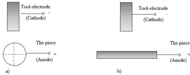
Figure 2. Schemes of electrode positioning used in the experimental investigations and their connection in the circuit of power impulse generator discharge: a) the case of cylindrical piece; b) the case of flat piece
