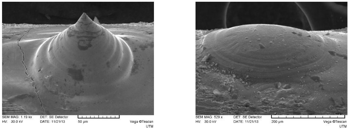
Figure 5. SEM images of Taylor cones that show growth of diameter of crater and of the base angle on reduction of current density. Power regimes: left - U=60 V, C=200 \mu F, d=0.2 mm, S=0.2 mm, right - U=70 V, C=200 \mu F, d=0.25 mm, sc=0.2 mm
