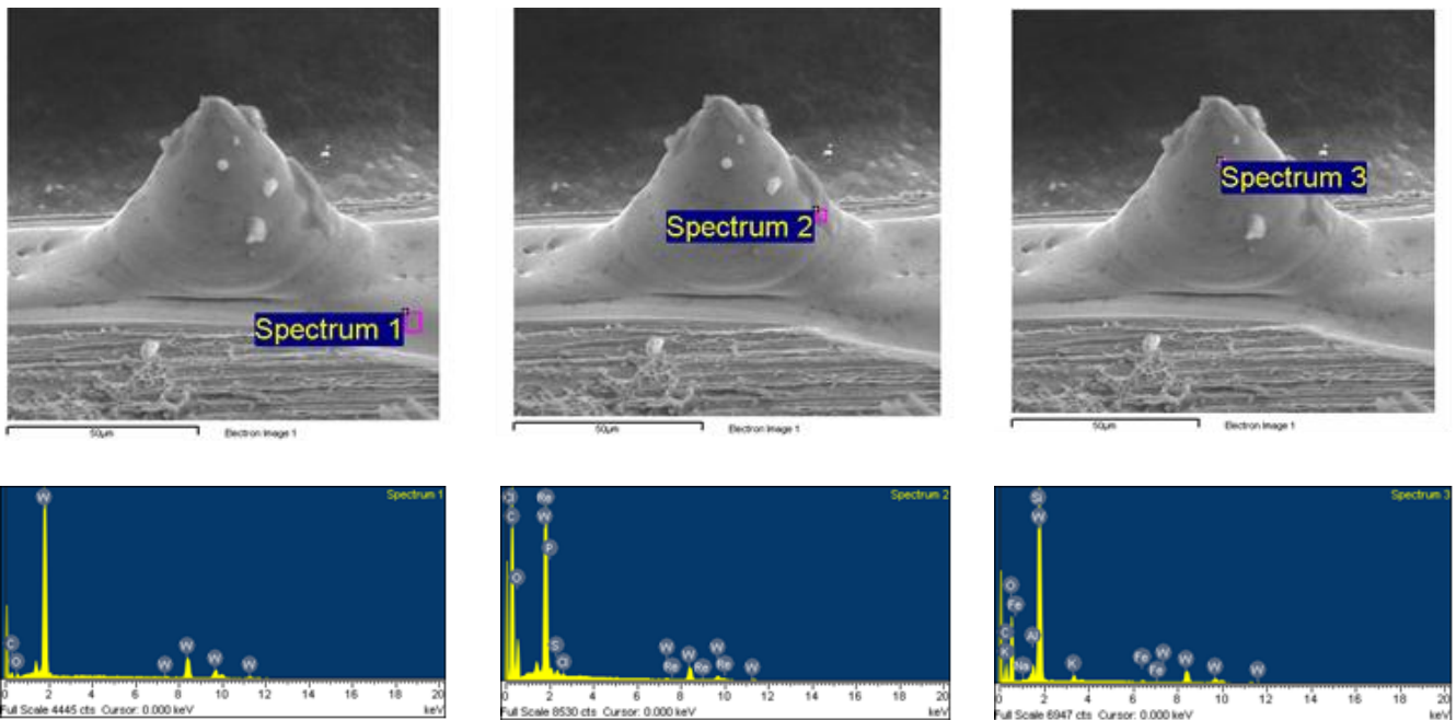
Figure 7. Results of EDX investigation of unprocessed plane sample made of W+10 % Re
