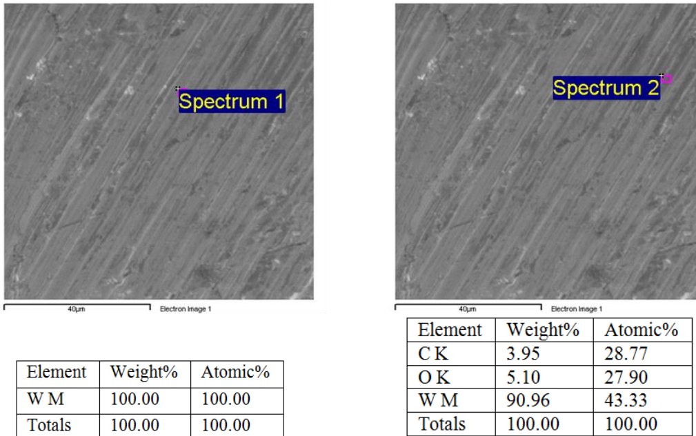
Figure 7. Results of EDX investigation of unprocessed plane sample made of W+10 % Re
