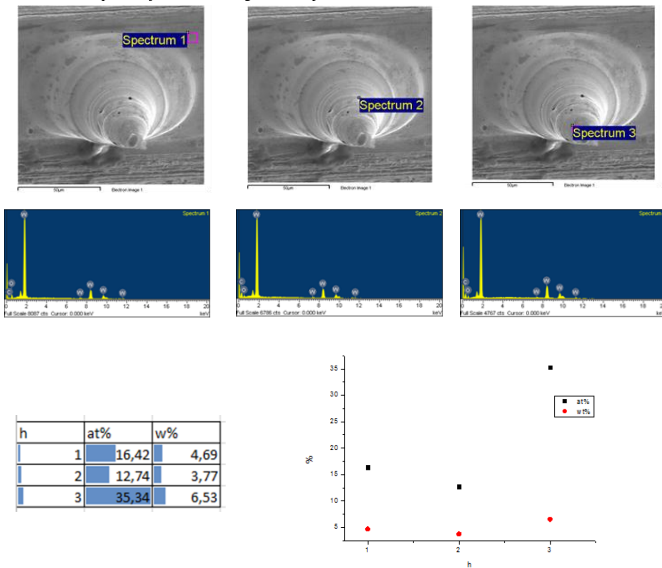
Figure 9. Results of EDX investigation of Taylor cones extracted on anode sample with power regime: U=60 V, C=200 \mu F, d=0.2 mm, S=0,2 mm for the first discharge and S=2 mm for the second discharge, where h1 – top, h2 – lateral surface, h3 – crater.
