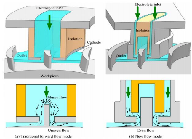
Figure 14. Illustrations of the flow method in the electrochemical treppanning [21]
